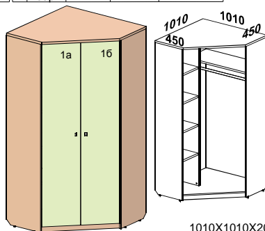
1010X1010X2065
