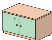
900X600X535
